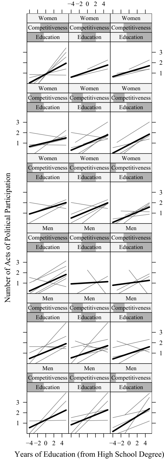
Figure 4: CONDITIONING WITH TWO CONTINUOUS VARIABLES USING SHINGLES. Within-state individual level outlier resistant regressions of participation on education are shown in gray. Black lines show the averages of the gray lines, weighted by the sample sizes of each state. Panel order is (a) low to high state level education going left to right — the part of the Education scale portrayed in each plot is shown by the shaded bars labeled “Education” and then (b) very competitive to not very competitive Senate races from bottom to top — the part of the Competitiveness scale portrayed in each panel is shown by the shaded bars labeled “Competitiveness”. The bottom three rows show the results for men and the top three rows show the results for women.
