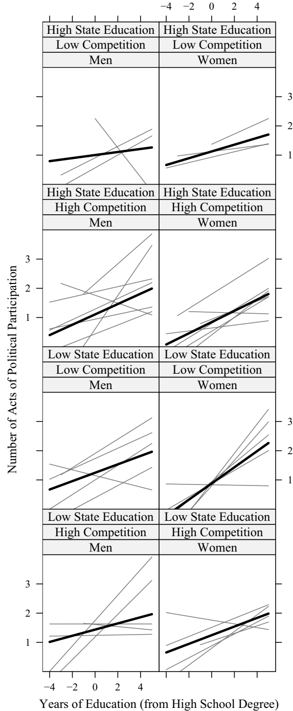
Figure 3: WITHIN-STATE OUTLIER-RESISTENT REGRESSIONS GROUPED BY LEVELS OF STATE-LEVEL EDUCATIONAL CONTEXT. The thin gray lines show the within-state, outlier-resistant regressions (MM-estimates) grouped by (1) gender of the respondent, (2) competitiveness of the state Senate Race (less than or equal to 25 percentage points difference=“high competition”, greater than 25 percentage points difference=“low competition”), and (3) percent of the state population college educated (median split at 22.5% with a college degree or more). The thick black lines were generated from averaging the intercepts and the slopes of the gray lines, weighting the average by the sample sizes within state. Unweighted averages were not detectably different except for Men in High Education States where the Senate Races were not very competitive.
