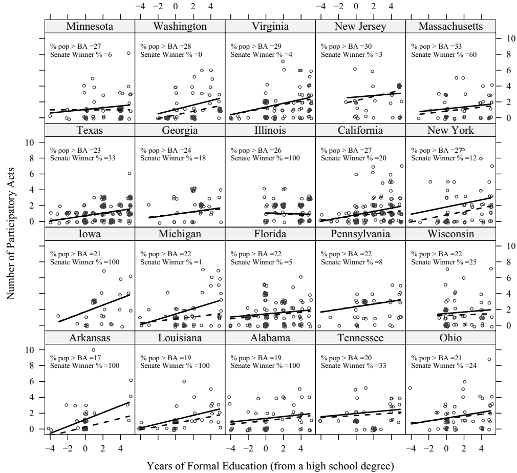
Figure 2: PARTICIPATION VERSUS EDUCATION WITHIN STATES Points are slightly jittered to show density. Education less than 8 years is coded as “-4”, 12 years of education is coded as “0”, education more than 16 years is coded as “5”. The solid straight lines is from OLS. The dashed straight line is from an outlier resistant linear model.
