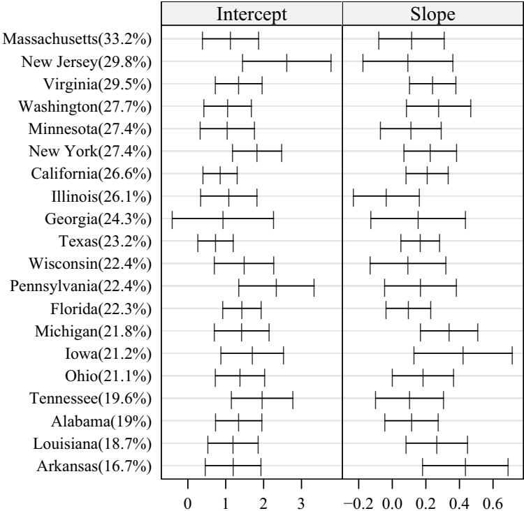
Figure 1: THE BETWEEN-STATE VARIATION OF WITHIN-STATE REGRESSIONS. The within-state regression estimates and 95% confidence intervals for the intercept and slope of education from equation 10 are plotted in order of state level education (percent of the state population aged 25-64 who have at least a college degree).
